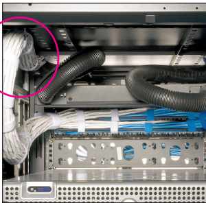
Cinch Tie mounted within cabinet UGCTC3S-X10
