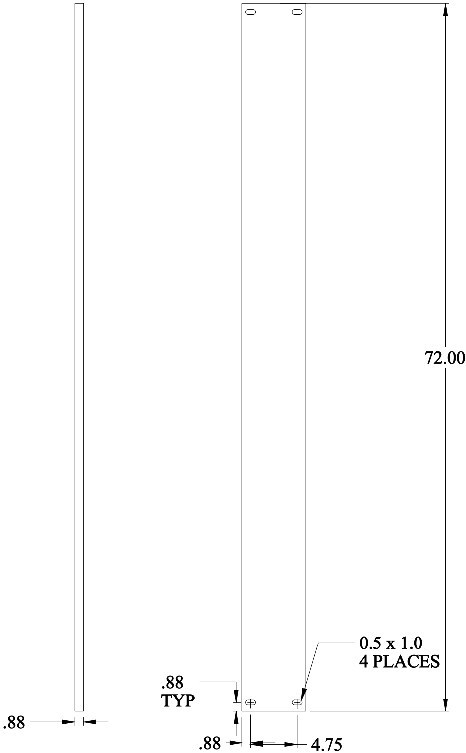
FORMED VIEW
