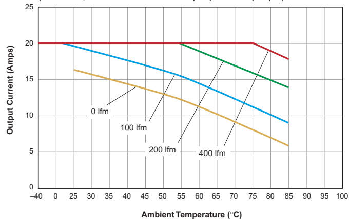
ULQ-3.3/20-D48
