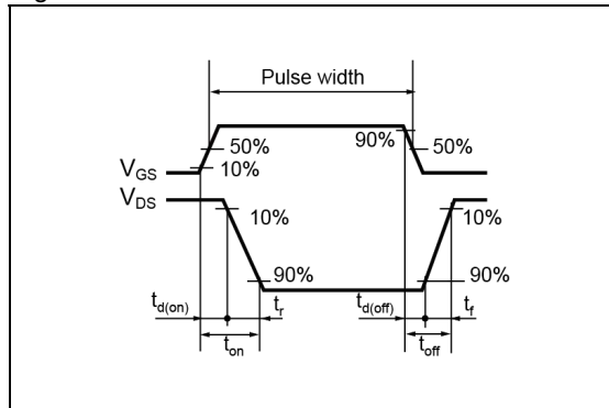
Fig. 1-2 SWITCHING WAVEFORMS
