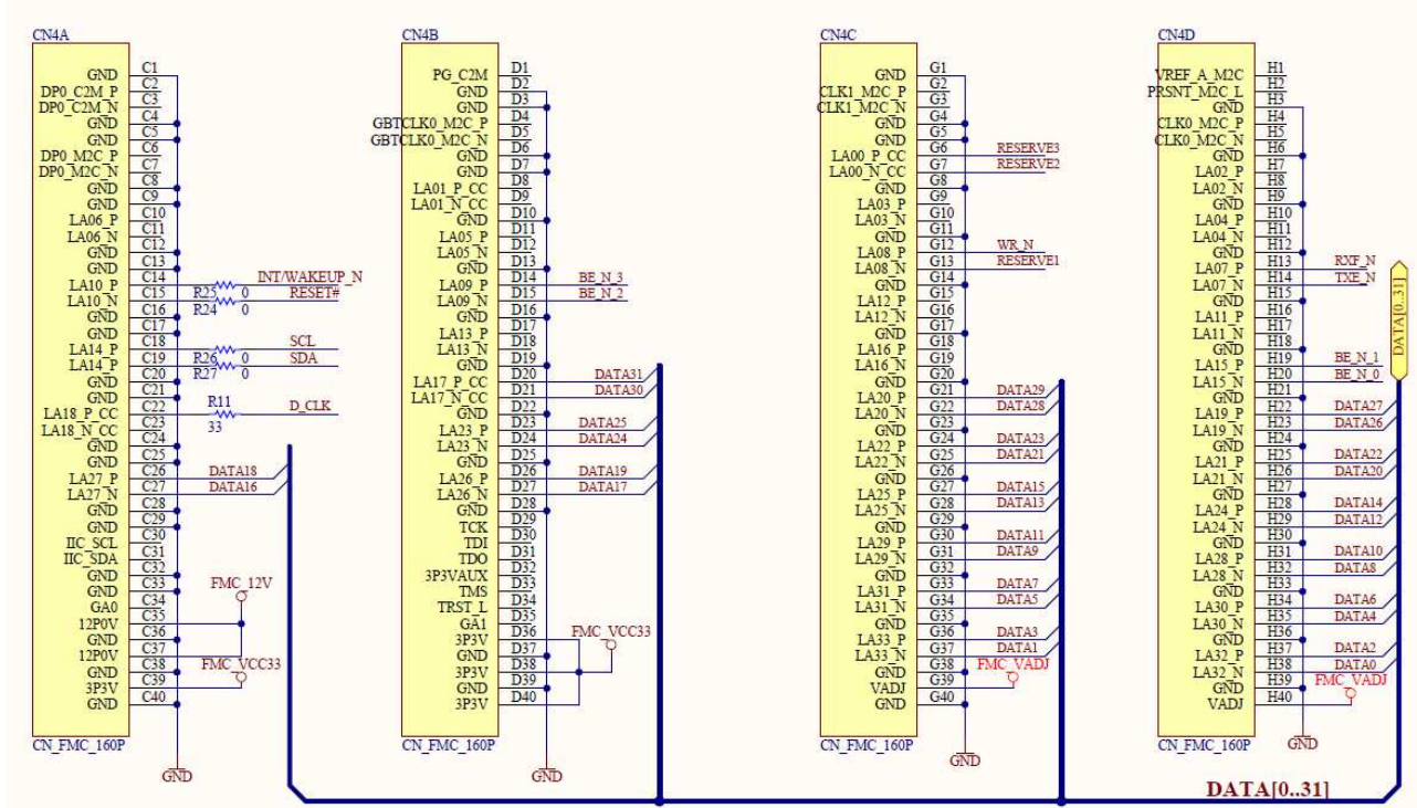
Figure 3-4 Schematics: FMC_UMFT602X
