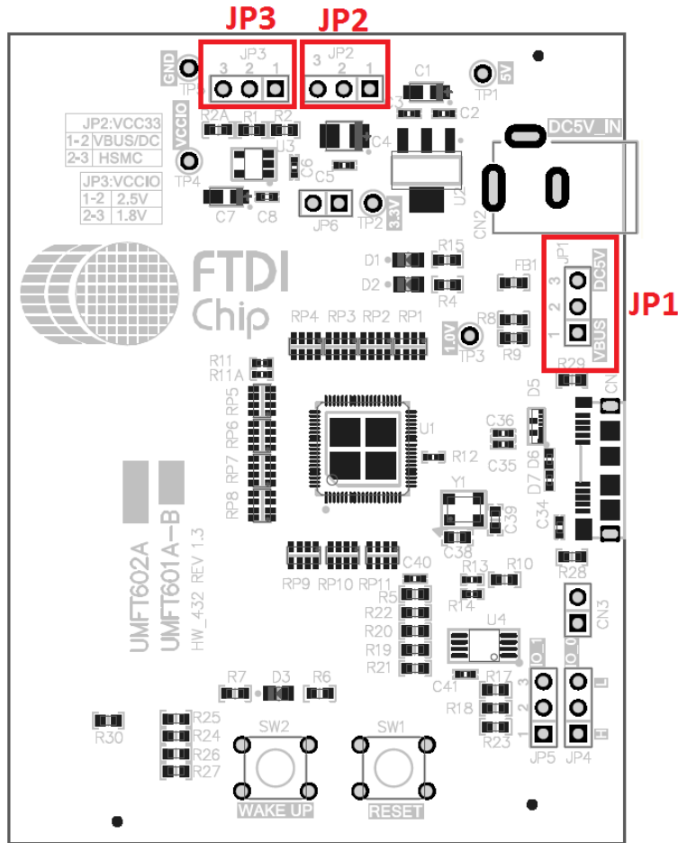
Figure 4-1 Jumpers Locations
