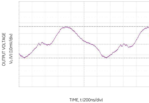
Figure 21. Typical output ripple and noise ( C_o=1 \times 47 \mu F ceramic, V_{IN} = 12V , I_o = I_{o,max} ).
