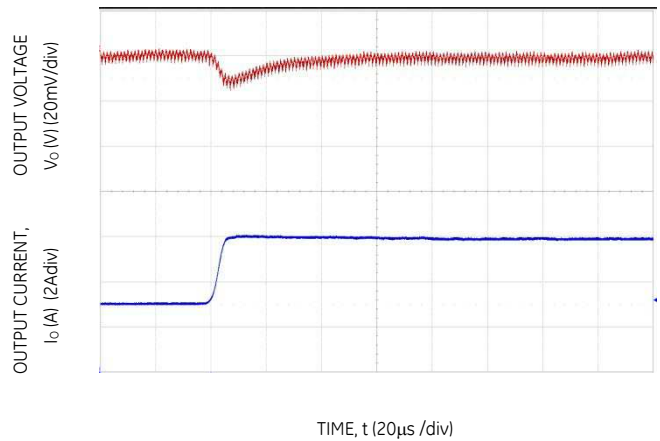
Figure 4. Transient Response to Dynamic Load Change from 50% to 100% at 12Vin, Cout=3x47µF+3x330µF, CTune=15nF, RTune=200Ω
