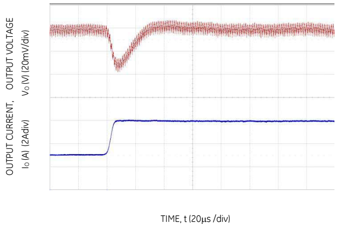
Figure 16. Transient Response to Dynamic Load Change from 50% to 100% at 12V in , C out = 2x47uF+1x330uF, CTune=2700pF & RTune=300Ω
