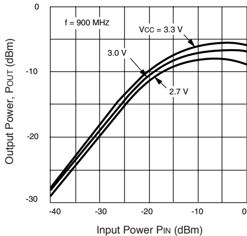
UPC2747TB OUTPUT POWER vs. INPUT POWER AND VOLTAGE
