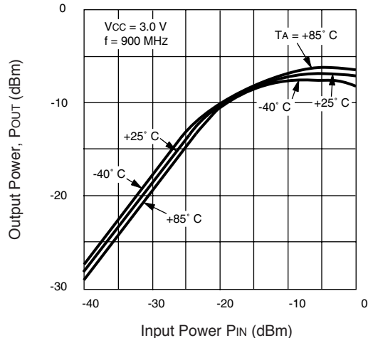
UPC2747TB OUTPUT POWER vs. INPUT POWER AND TEMPERATURE
