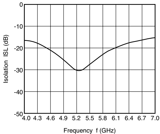
RX-TX ISOLATION vs. FREQUENCY (When ANT2-RX is ON)
