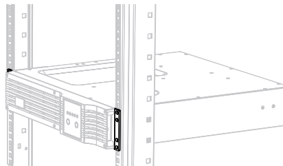
4-Post Rackmount
