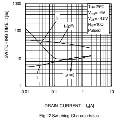
Fig.12 Switching Characteristics
