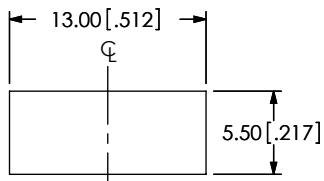
SUGGESTED PANEL CUTOUT DIMENSIONS
