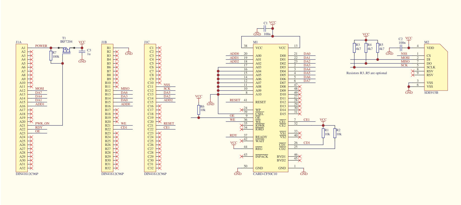
Figure 14. CF, MMC, SD Memory Expansion Board (AB5) - Schematic
