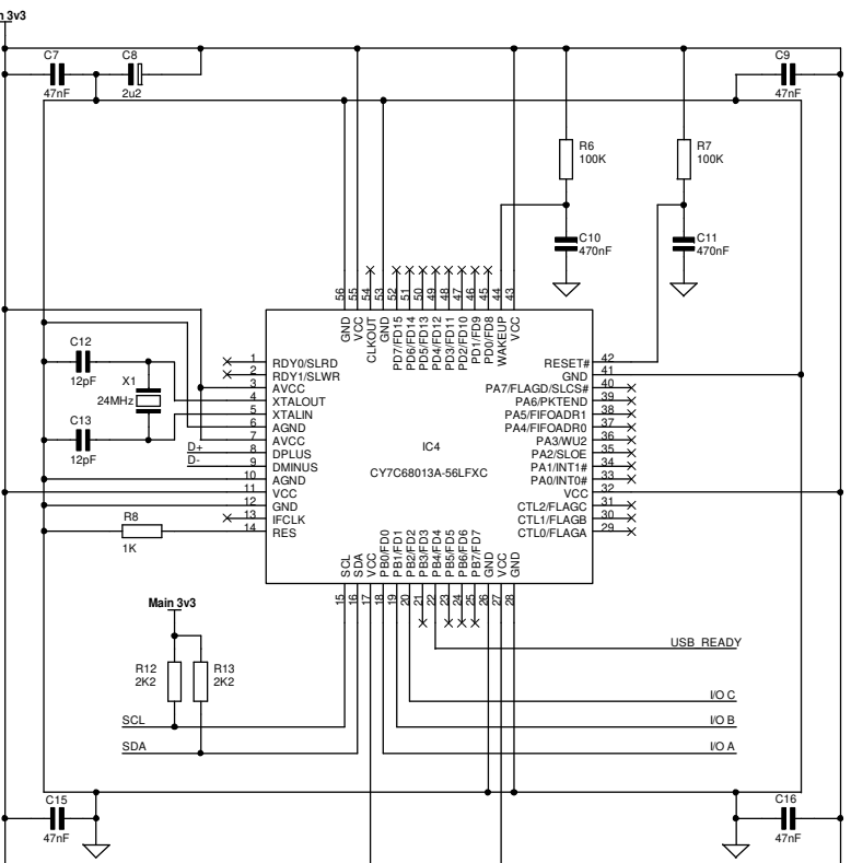
Figure 2. USB-to-I 2 C Interface Dongle Schematic Rev. 0 | Page 3 of 4
