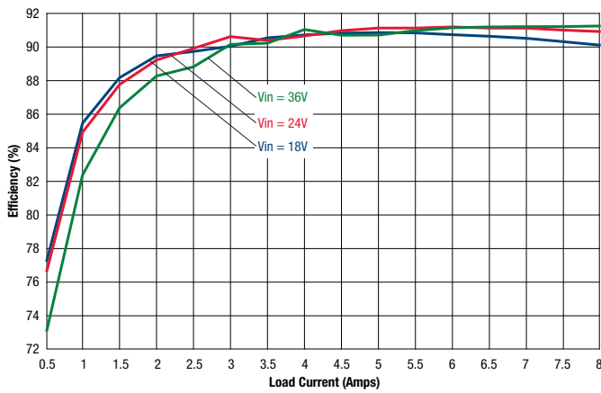
Efficiency vs. Line Voltage and Load Current @ 25°C – Vin = 18V-36V
