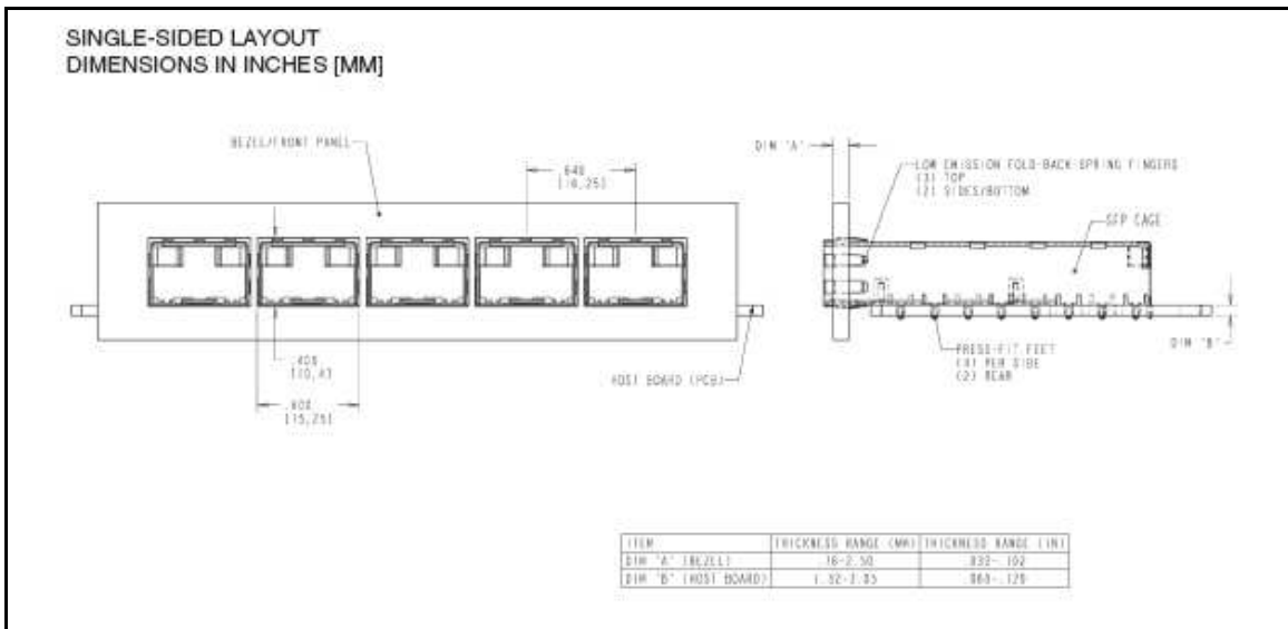
Figure 2 Single-sided Layout
