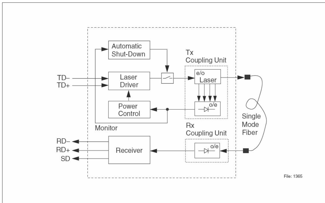
Figure 2 Functional Diagram
