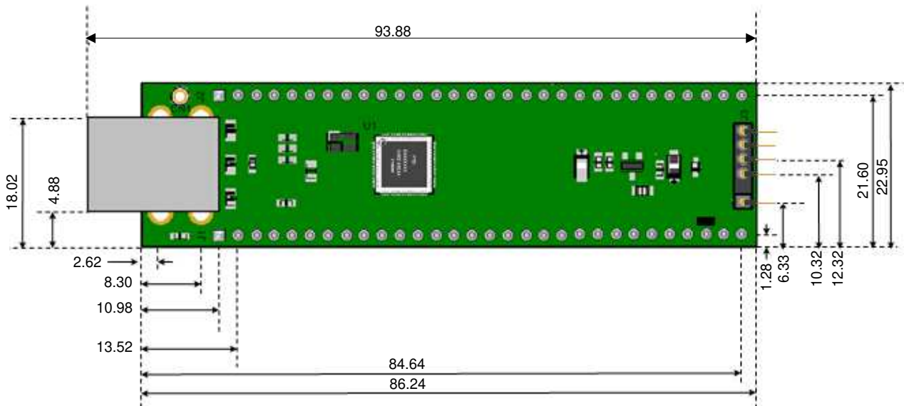
Figure 5.1 - V2DIP2 -64 Dimensions (Top View)
