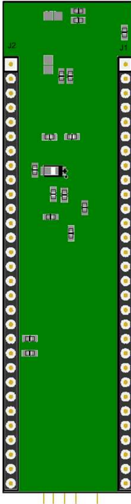
Figure 3.2 - V2DIP2-64 Module Pin Out (Bottom View)
