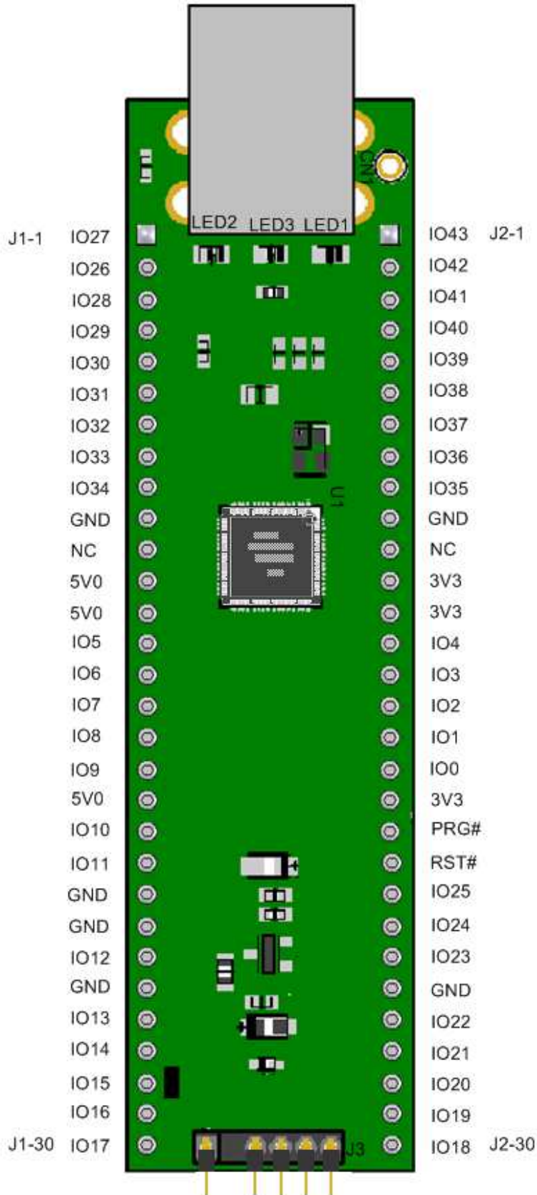
Figure 3.1 - V2DIP2-64 Module Pin Out (Top View)
