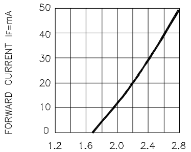
FORWARD VOLTAGE(Vf)-VOLTS
