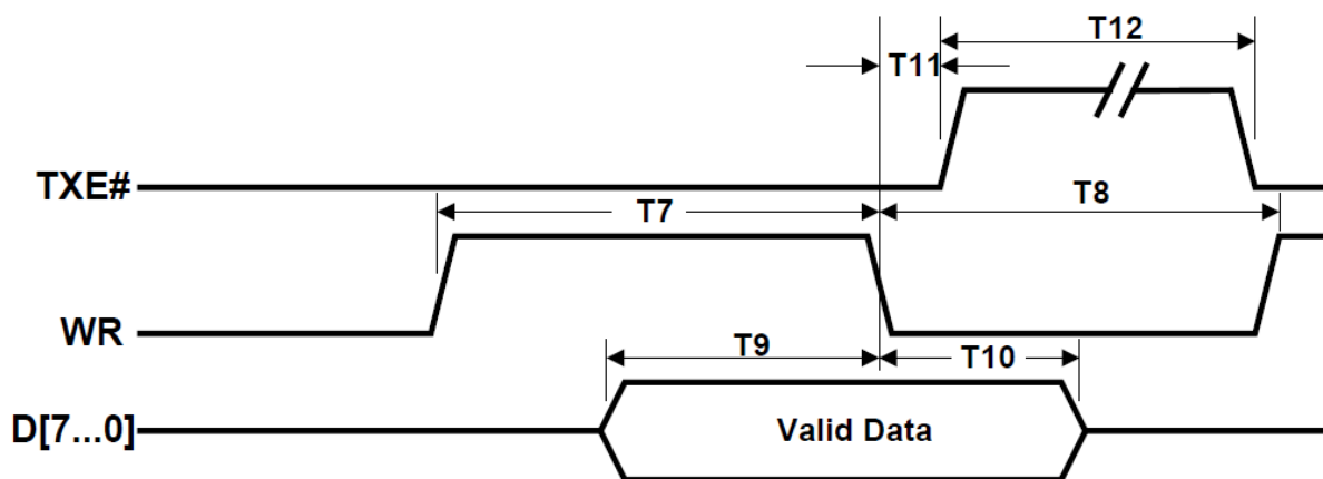
Figure 3.7 - FIFO Write Cycle.
