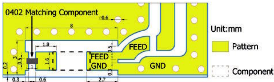
Land Pattern
