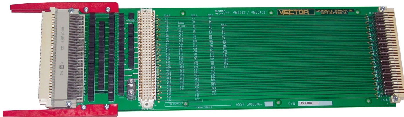
3U, VME64x J2 with 5-row, 160 positions DIN 41612 style connectors (click on image to enlarge)
