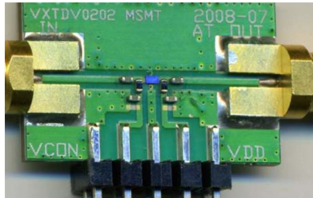
Figure 8. VMMK-3113 Charaterization Board
