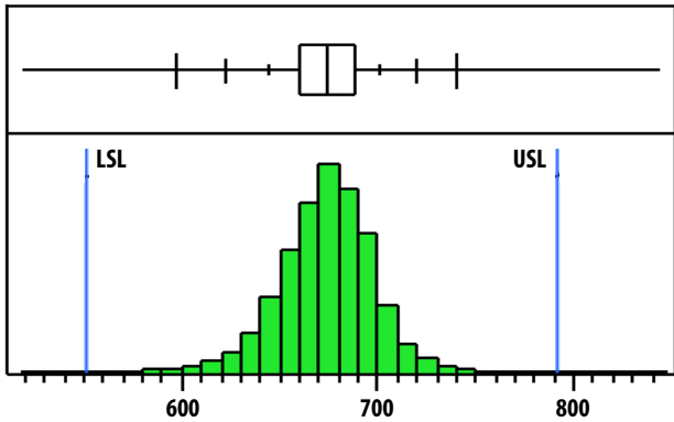
Vdet_On @ Pin = +12 dBm: Mean = 674 mV, LSL = 550 mV, USL = 790 mV
