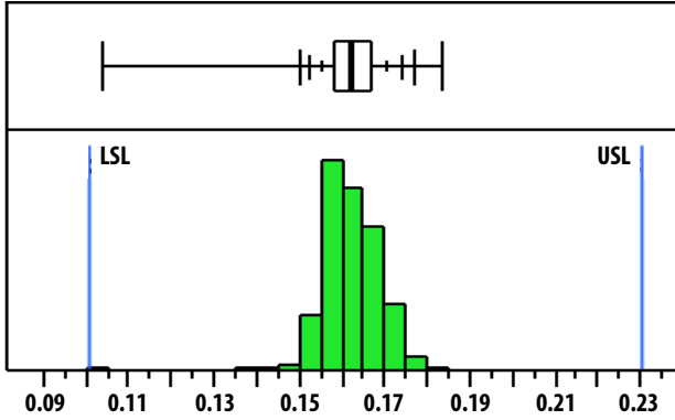
Ibias: Mean = 0.16 mA, LSL = 0.1 mA, USL = 0.23 mA
