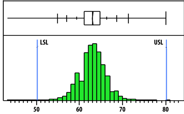
Voffset: Mean = 63 mV, LSL = 50 mV, USL = 80 mV
