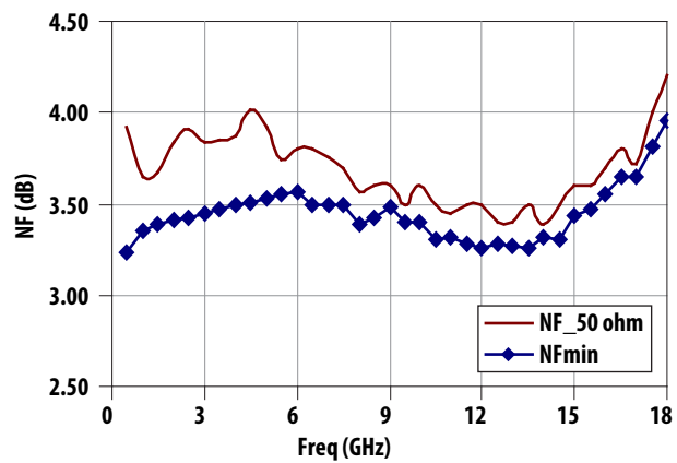
Figure 6. Noise Figure ( V_c = 1.8\text{V} )
