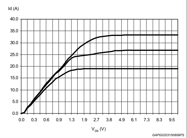
Figure 23. Output characteristics
