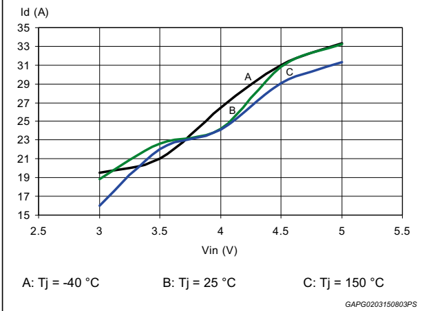
Figure 22. Transfer characteristics
