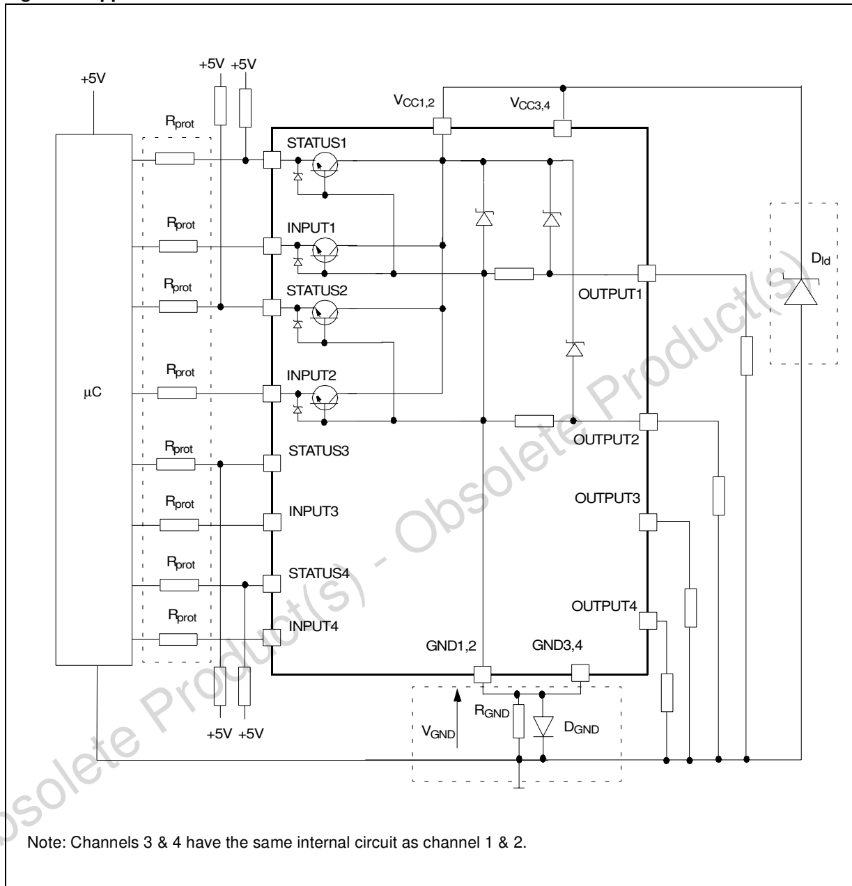
Figure 8. Application Schematic
