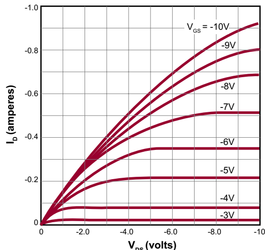
Saturation Characteristics
