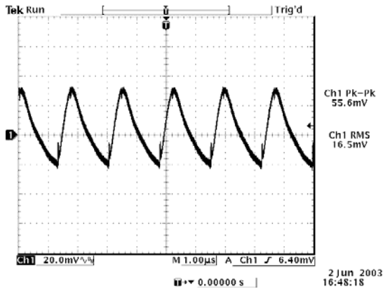
3.3 Vdc input, 12 Vdc output
