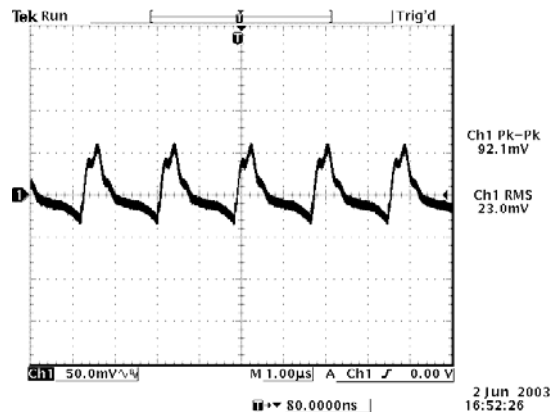
3.3 Vdc input, 15 Vdc output
