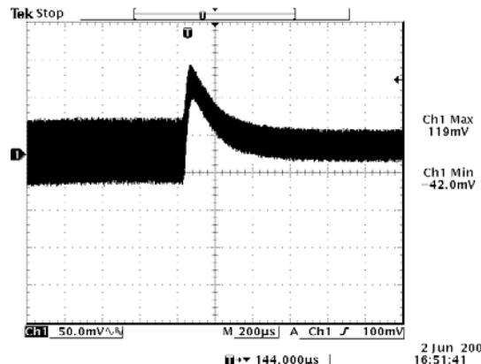
100% to 50% load transient at V_{in}=3.3 V, V_o=15 V
