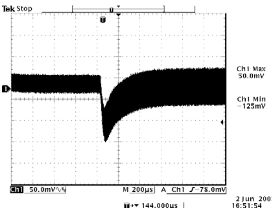
50% to 100% load transient at V_{in}=3.3 V, V_o=15 V
