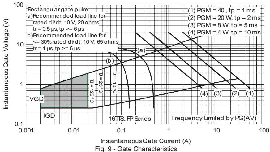
Fig. 9 - Gate Characteristics
