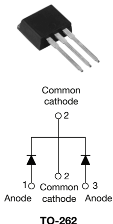
VS-43CTQ...G-1
