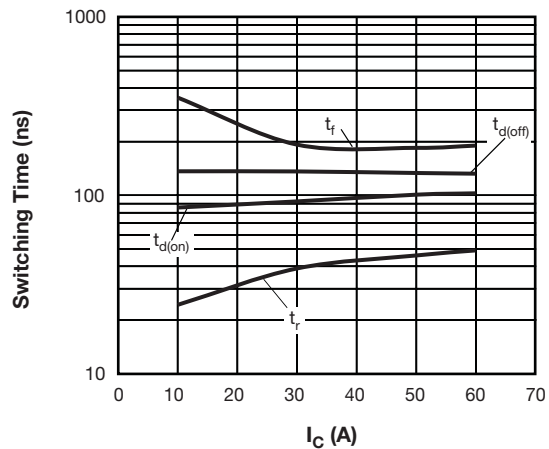
Fig. 8 - Typical Q1 - Q4 Trench IGBT 1200 V Switching Time vs. I_C (with D1 - D4 Freewheeling Diode), T_J = 125\text{ }^\circ\text{C} , V_{CC} = 600\text{ V} , R_g = 4.7\ \Omega , V_{GE} = 15\text{ V} , L = 500\ \mu\text{H}
