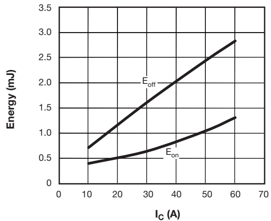
Fig. 7 - Typical Q1 - Q4 Trench IGBT 1200 V Energy Loss vs. I_C (with D1 - D4 Freewheeling Diode), T_J = 125\text{ }^\circ\text{C} , V_{CC} = 600\text{ V} , R_g = 4.7\ \Omega , V_{GE} = 15\text{ V} , L = 500\ \mu\text{H}
