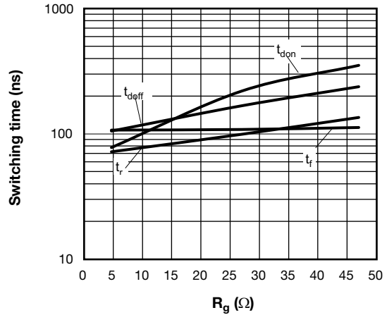
Fig. 10 - Typical Q1 - Q4 Trench IGBT Switching Time vs. R g (with D5 - D6 Clamping Diode) T J = 125 °C, V CC = 300 V, I C = 75 A, V GE = 15 V, L = 500 μH
