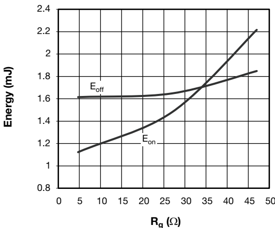
Fig. 9 - Typical Q1 - Q4 Trench IGBT Energy Loss vs. R g (with D5 - D6 Clamping Diode) T J = 125 °C, V CC = 300 V, I C = 75 A, V GE = 15 V, L = 500 μH
