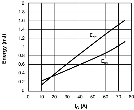
Fig. 7 - Typical Q1 - Q4 Trench IGBT Energy Loss vs. I C (with D5 - D6 Clamping Diode) T J = 125 °C, V CC = 300 V, R g = 4.7 Ω, V GE = 15 V, L = 500 μH
