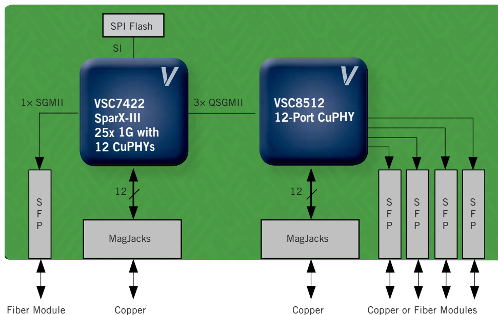
VSC7422 in a 25-port 1-GbE switch application
