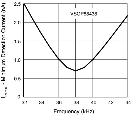
Fig. 4 - Bandpassfilter Characteristic
