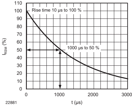
Fig. 1 - 10/1000 μs Peak Pulse Current Wave Form
