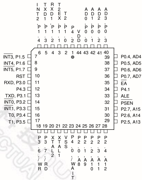
44-Pin PLCC
