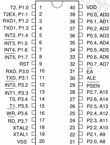
40-Pin DIP
