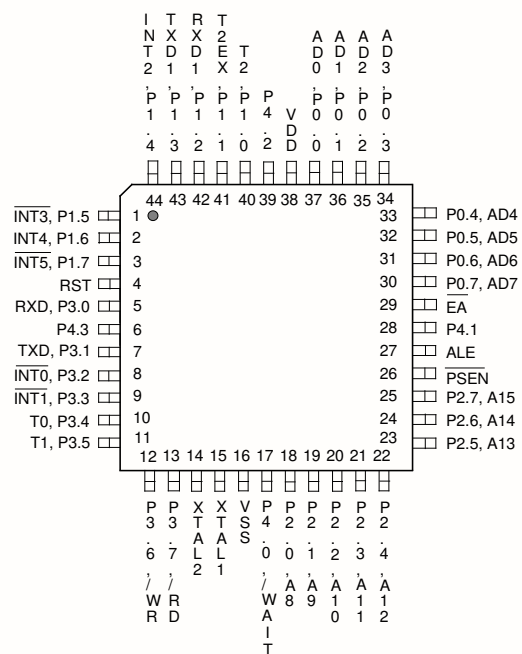
44-Pin QFP
