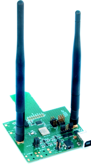
Evaluation Kit
