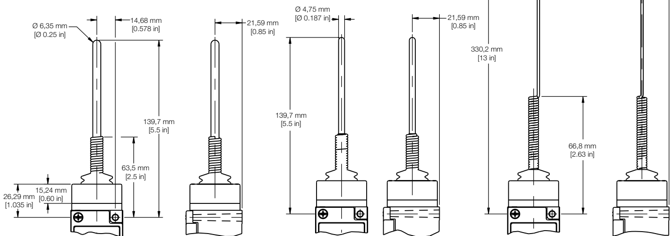
Figure 6. Limitless™ WLS Series Wobblers
