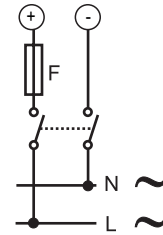
Fig. 19 Auxiliary power supply (H). 250 V [T] 630 mA fuse (F).
