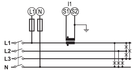
Fig. 7 Three-phase system with neutral (4-wire), unbalanced load, 1 CT. 315 mA fuse (F).
