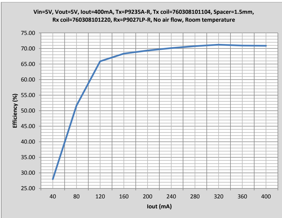
Figure 7. Typical Efficiency Curve for 20mm Coil
