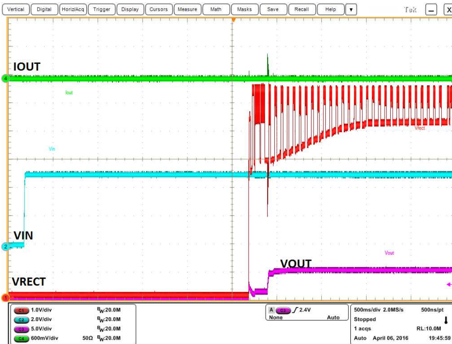
Figure 11. No Load Start-up by Tx Input Power (Ch1=Vrect, Ch2=VIN, Ch3=Vout,Ch4=Iout)
