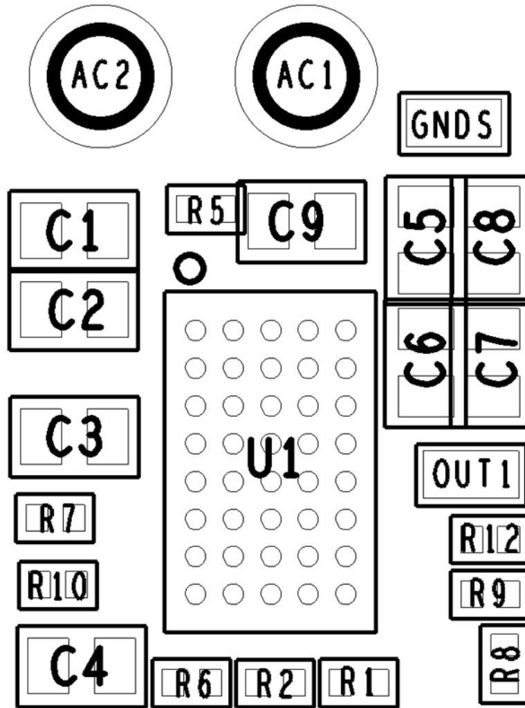
Figure 18. P9027LP-R-EVK Component Map
