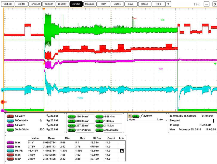
Figure 10. 0 to 400mA Step Load Response (Ch1=Vrect, Ch2=VSNS, Ch3=Vout, Ch4=Iout)
