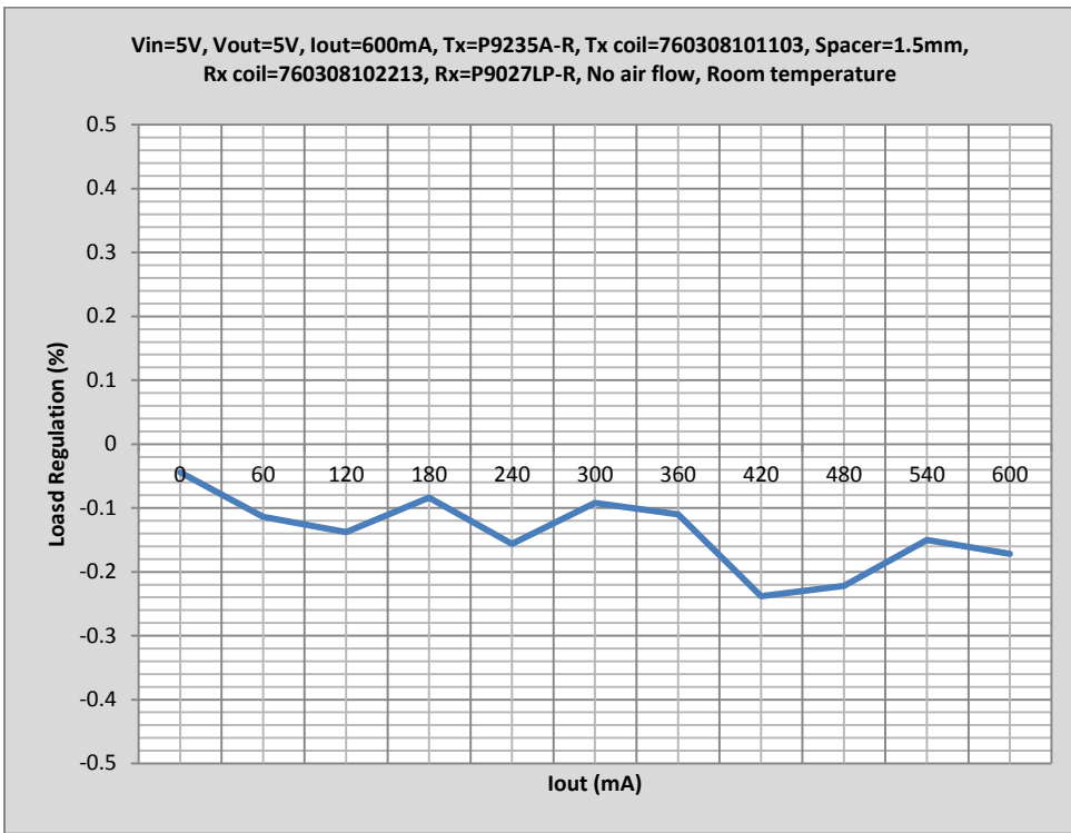
Figure 6. Load Regulation for 30mm Coil
