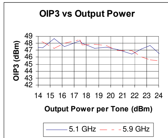
Figure 3 OIP3
