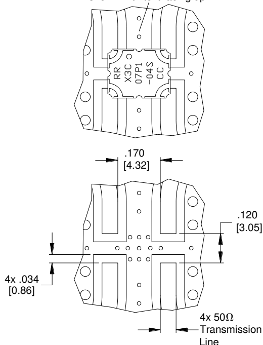
Dimensions are in Inches [Millimeters] X3C07P1-04S Mounting Footprint
