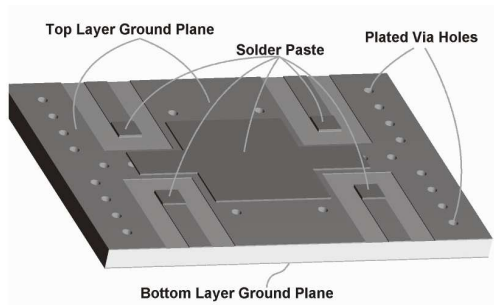
Figure 3: Solder Paste Application
