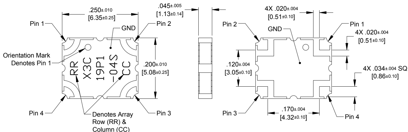
Dimensions are in Inches [Millimeters] X3C19P1-04S Mechanical Outline
