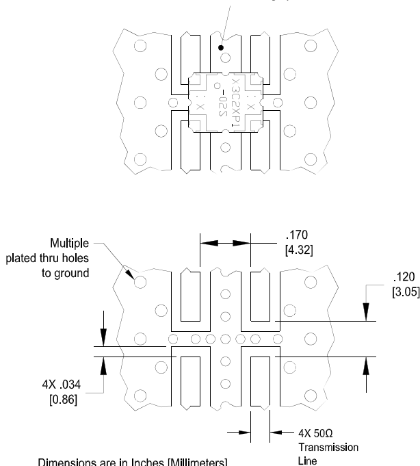
Dimensions are in Inches [Millimeters] X3C26P1-03S Mounting Footprint
