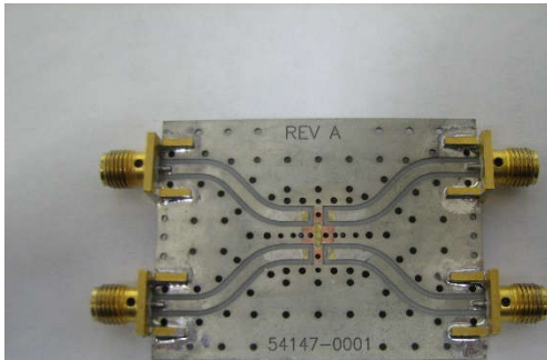
2, 3 dB and 5dB Test Board
