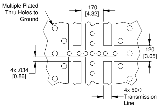
Dimensions are in Inches [Millimeters] X3C25P1-05S Mounting Footprint
