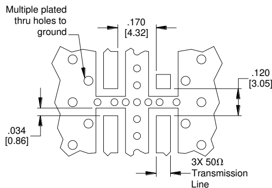
Dimensions are in Inches [Millimeters] X3DC23P1S Mounting Footprint
