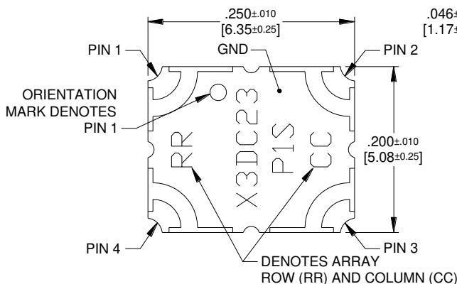
Dimensions are in Inches [Millimeters] X3DC23P1S Mechanical Outline
