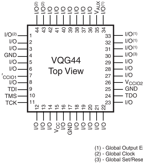
Figure 6: VQG44 Package
