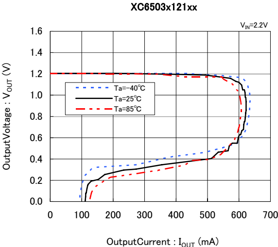
(1) OutputVoltage v.s. OutputCurrent
