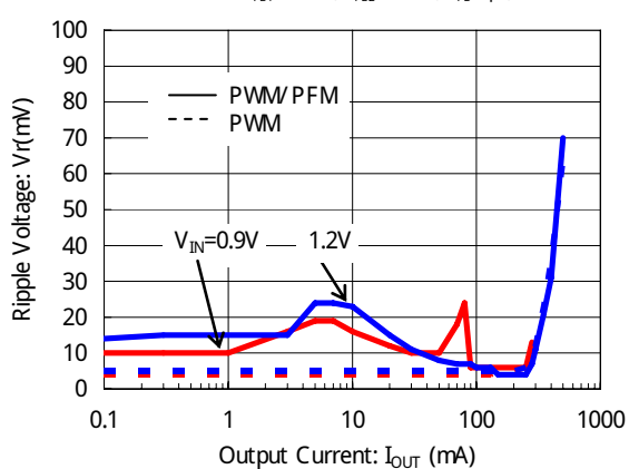
XC9131x05C (V OUT =1.8V)
