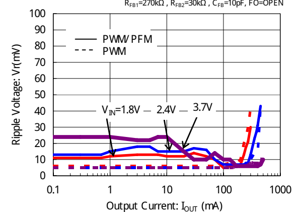
XC9131x05C (V OUT =5.0V)
